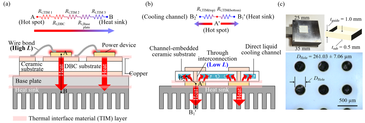
Figure 1. Ceramic substrate for hybrid dual-side cooling power device module. (a) Conventional power device module with wire bonding connection using single-side cooling. (b) Proposed power device module packaging employing 3D-printed channel embedded ceramic through-hole substrate using dual-side cooling with heat sink and direct liquid cooling channel. (c) Optical images of 3D-printed ceramic substrate with through holes for vertical interconnection.
